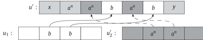
Fig. 4. Inserting a^n again....
