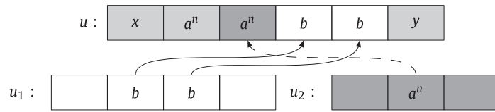
Fig. 3. Case a^n in u_2 .
