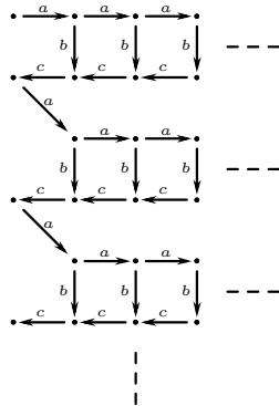
Figure 3.15. Transformation of Theorem 3.12.
