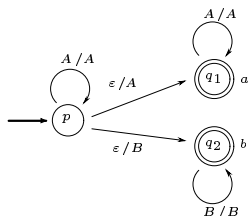
Figure 2.2: Transducer recognizing the grid
