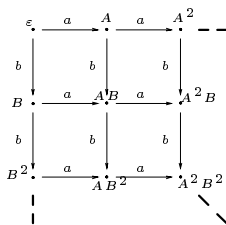
Figure 2.1: The grid, with vertices in \{A, B\}^*
