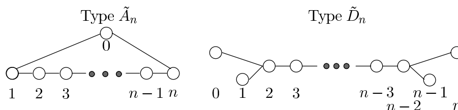
FIGURE 8. The Dynkin diagrams of type \tilde{A}_n and \tilde{D}_n
