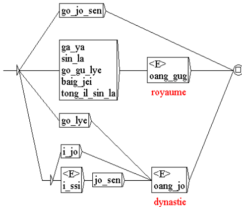
Figure 68 : Graphe Ndyn
