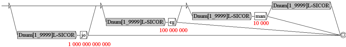
Figure 18 : Graphe DnumAll-SICOR
