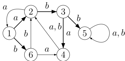
Fig. 2. A transition structure on a 2-letters alphabet having 1 as initial state
