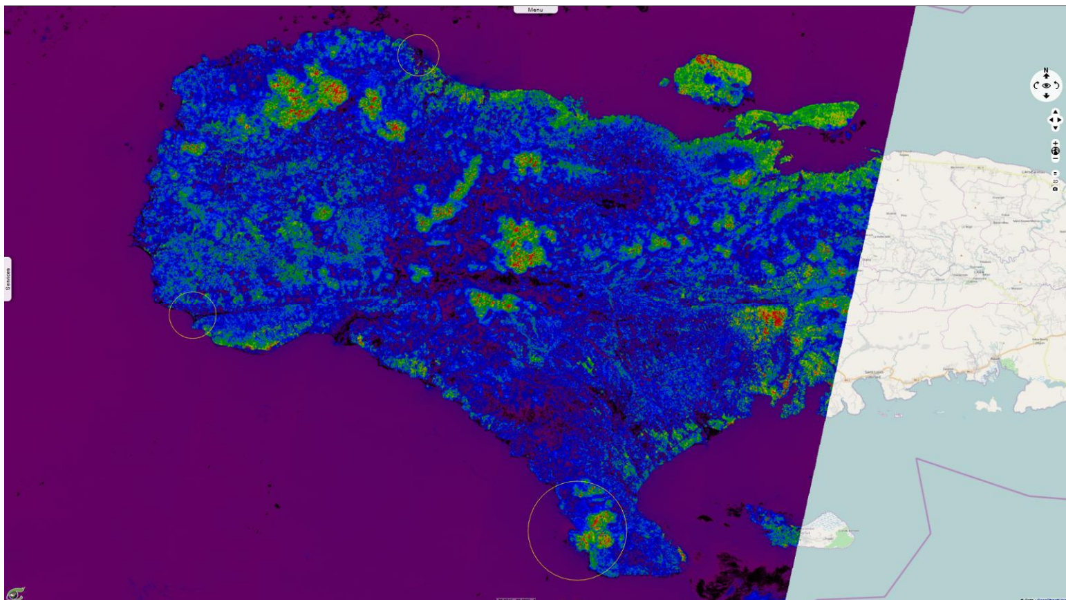
L8 04.11.2016 (after) - Normalized Difference Infrared Index (5 vs.6, [0;0.4]) 2D view
