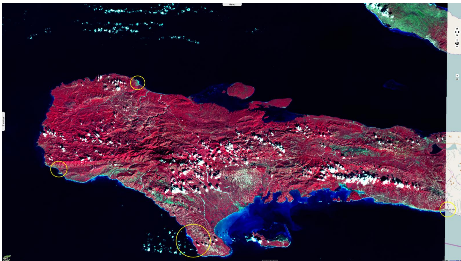
S2 24.12.2015 (before) - Near-infrared colour composition (8-4-3) 2D view
