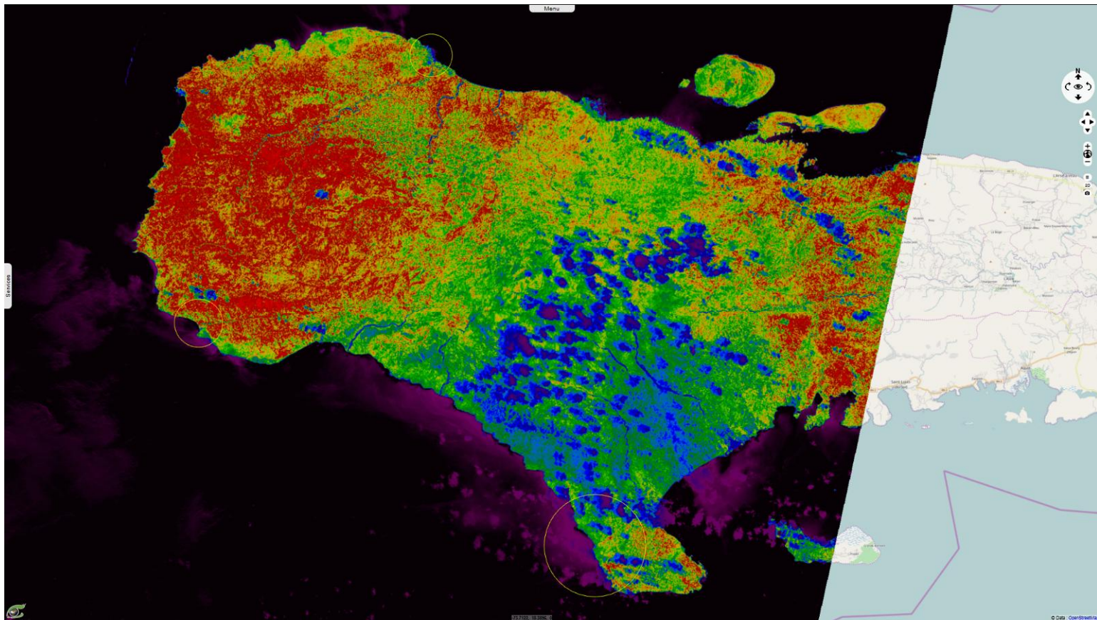
L8 01.09.2016 (before) - Normalized Difference Vegetation Index (5 vs.4, [0;0.6]) 2D view
