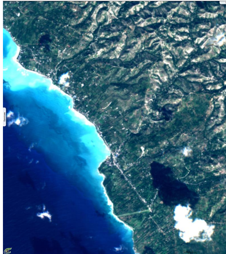
S2 24.12.2015 (left) vs. S2 09.10.2016 (right) - Natural colour composition (4-3-2) 2D animation
