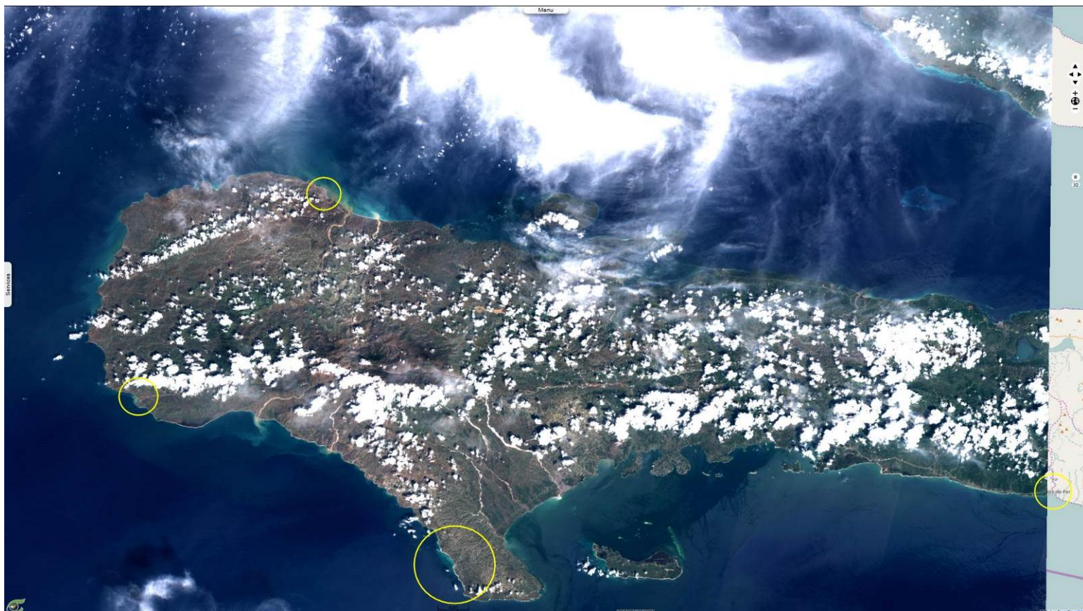
S2 09.10.2016 (after) - Natural colour composition (4-3-2) 2D_view
