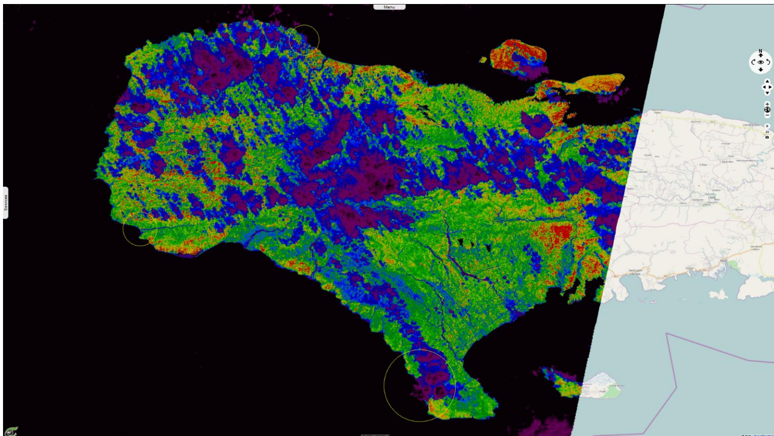
L8 04.11.2016 (after) - Normalized Difference Vegetation Index (5 vs.4, [0;0.6]) 2D view
