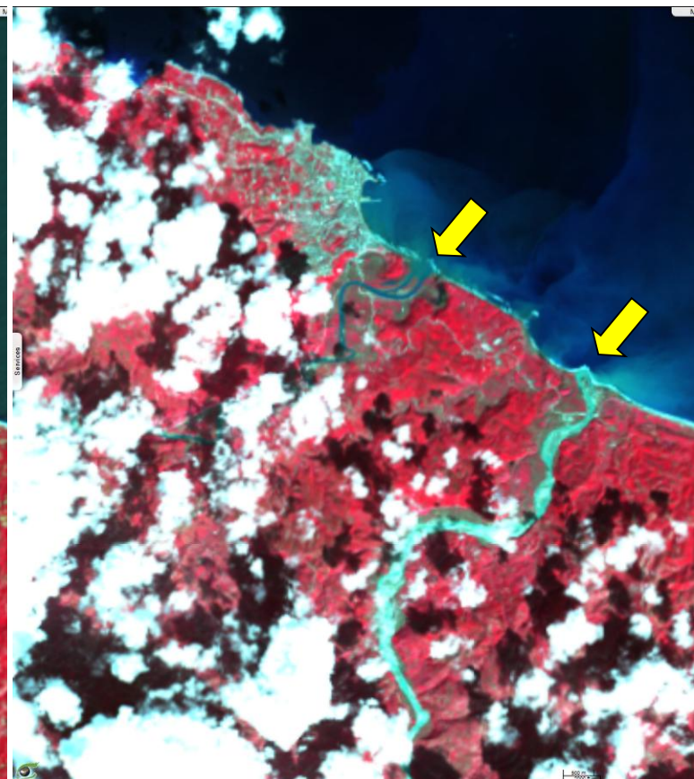
L8 01.09.2016 (left) vs. L8 04.11.2016 (right) - Near-infrared colour composition (5-4-3) 2D animation
