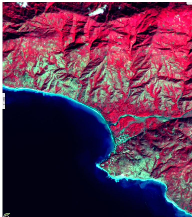
S2 24.12.2015 (left) vs. S2 09.10.2016 (right) - Near-infrared colour composition (8-4-3) 2D animation
