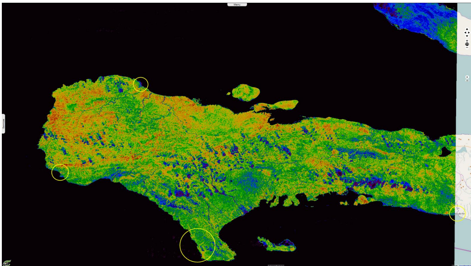
S2 24.12.2015 (before) - Normalized Difference Vegetation Index (8 vs.4, [0;1] - 10m) 2D_view
