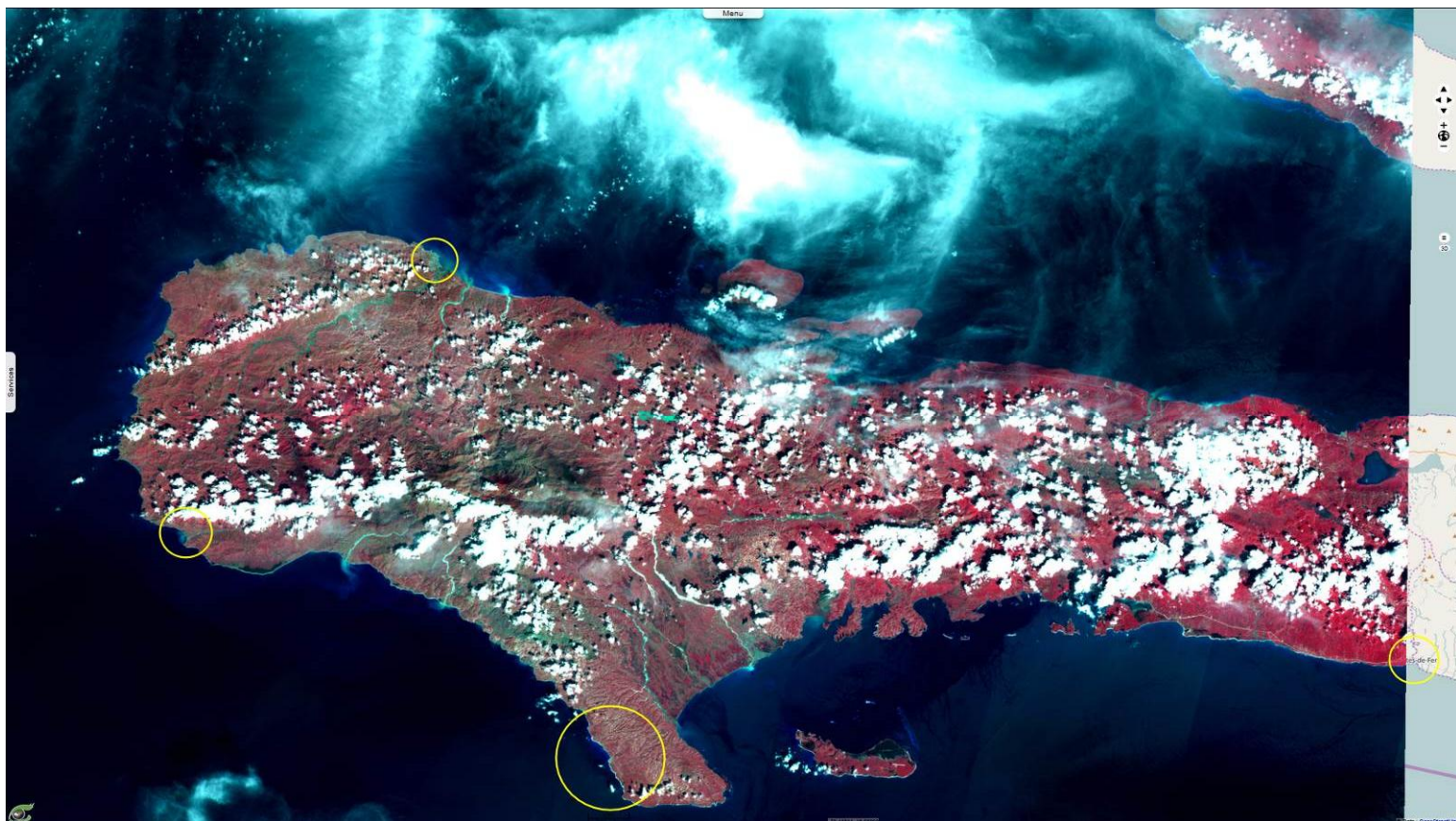
S2 09.10.2016 (after) - Near-infrared colour composition (8-4-3) 2D view
