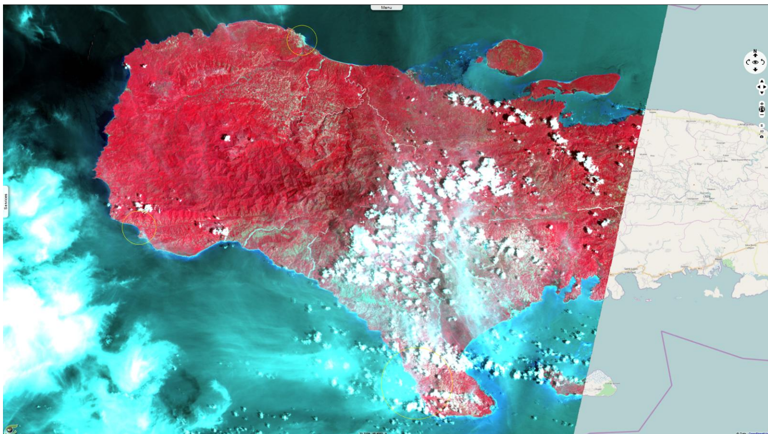
L8 01.09.2016 (before) - Near-infrared colour composition (5-4-3) 2D view
