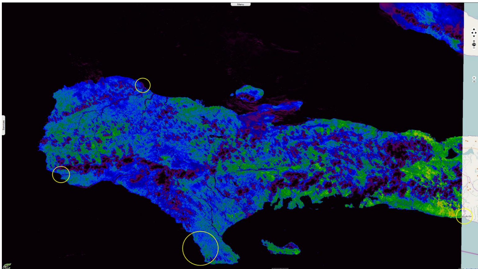
S2 09.10.2016 (after) - Normalized Difference Vegetation Index (8 vs.4, [0;1] - 10m) 2D_view
