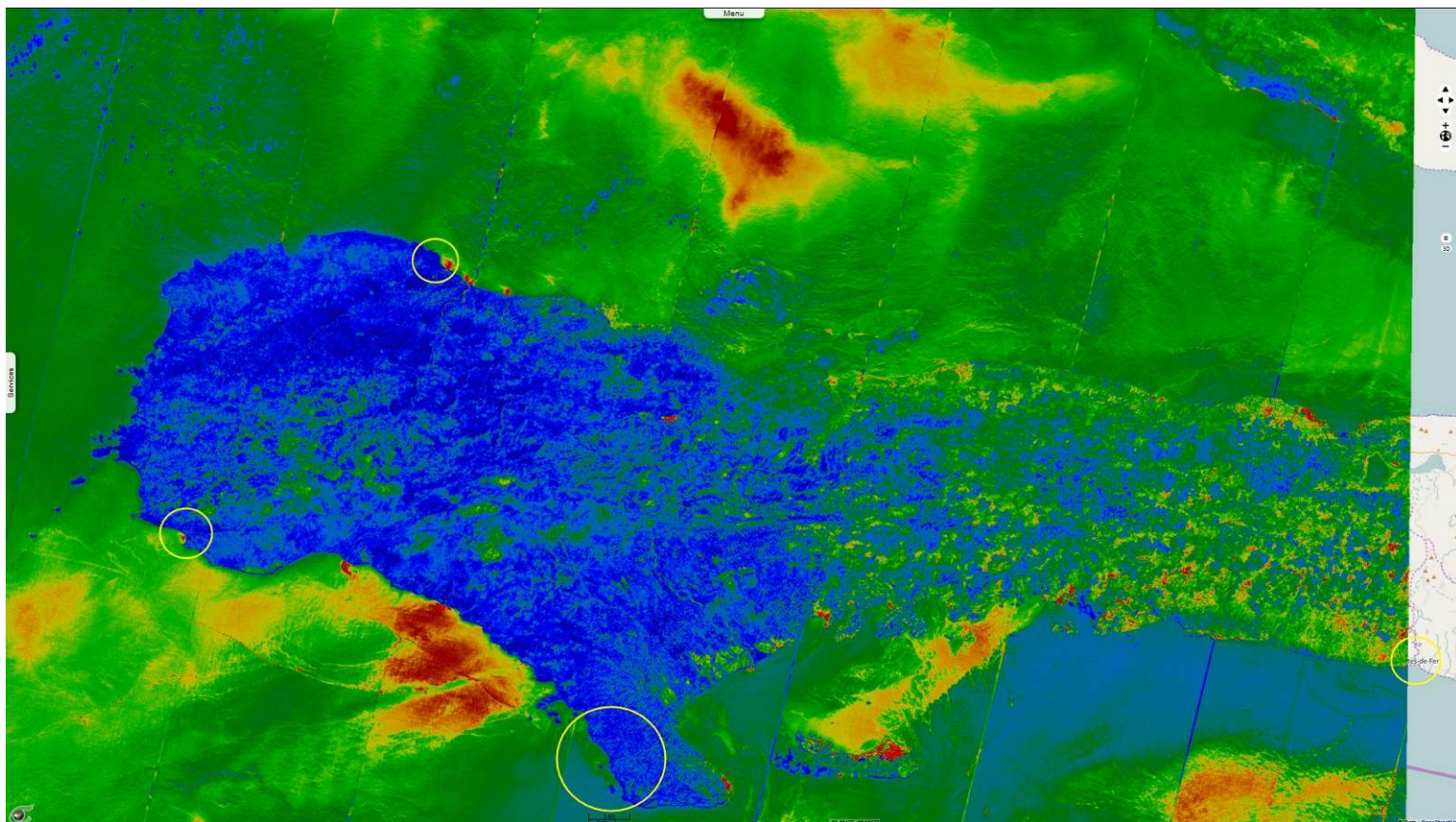
S2 09.10.2016 (after) - Normalized Difference Infrared Index (8 vs.11, [-0.2;0.6] - 20m) 2D view
