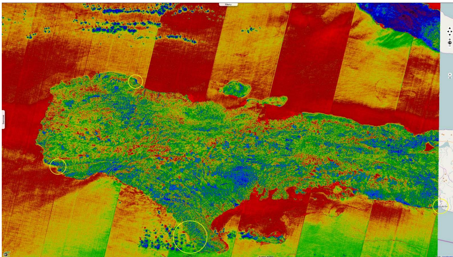
S2 24.12.2015 (before) - Normalized Difference Infrared Index (8 vs.11, [-0.2;0.6] - 20m) 2D view
