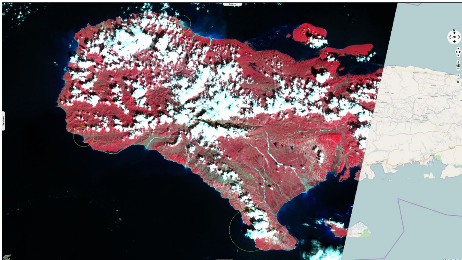
L8 04.11.2016 (after) - Near-infrared colour composition (5-4-3) 2D view
