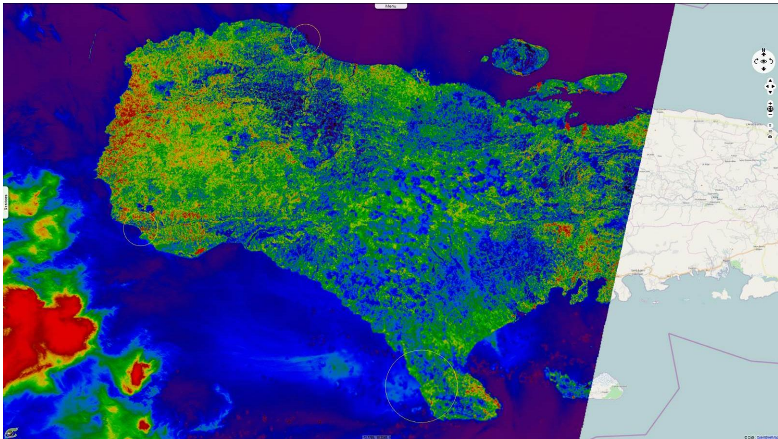
L8 01.09.2016 (before) - Normalized Difference Infrared Index (5 vs.6, [0;0.4]) 2D view
